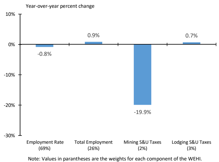
► Figure 3: Change in Components of WEHI - January 2025
